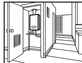
Closest installation of Model 1600H with proper ventilation shown.
